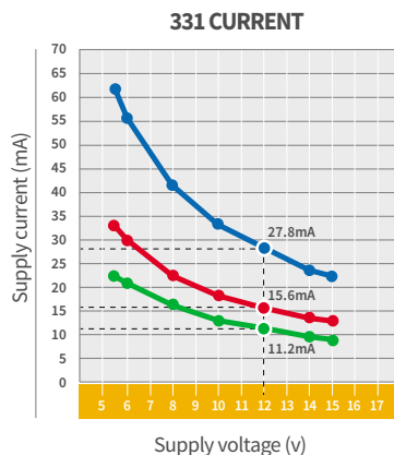
FIG 1: SUPPLY CURRENT VS. SUPPLY VOLTAGE
